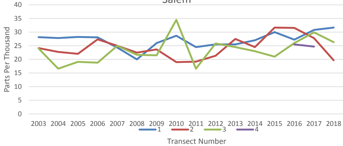
Average Salinity at Set 3 (No Phragmites) Wells, Forest River Salem
