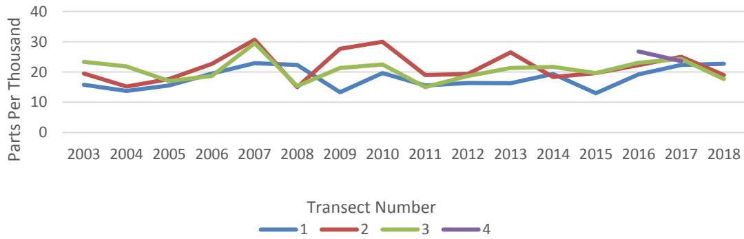
Average Salinity at Set 2 (Transition between Phragmites and salt marsh grasses) Wells, Forest River Salem
