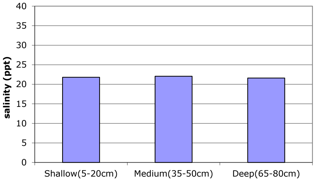
Salem Forest River 2003-2018 Average Salinity vs. Well Depth
