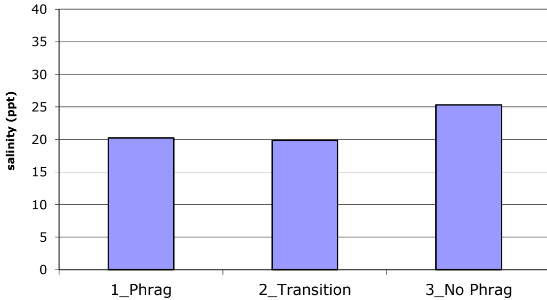
Forest River, Salem, 2003-2018 Average salinity vs. presence of Phragmites
