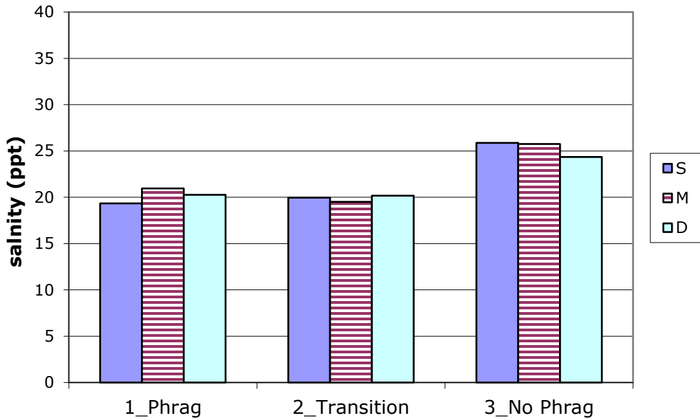
Forest River, Salem, 2003-2018 Average salinity vs. depth and presence of Phragmites
