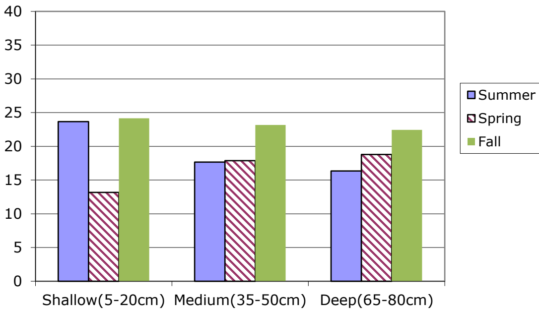
Salem Forest River 2003-2018 Seasonal Average Salinity vs. Well Depth
