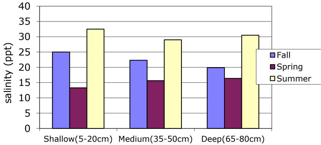
Littleneck Rd., Ipswich 1999-2018 Seasonal Average Salinity vs. Well Depth
