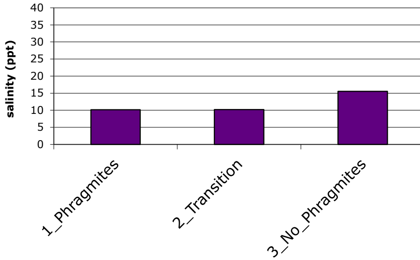
Railroad Ave., Rowley 1997-2011 Average Salinity vs. Presence of Phragmites
