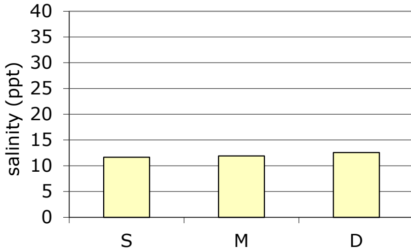
Railroad Ave., Rowley 1997-2011 Average Salinity vs. Well Depth
