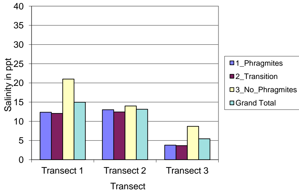
Average salinity by vegetation type, Batchelder's Landing Rowley, 1996-2011
