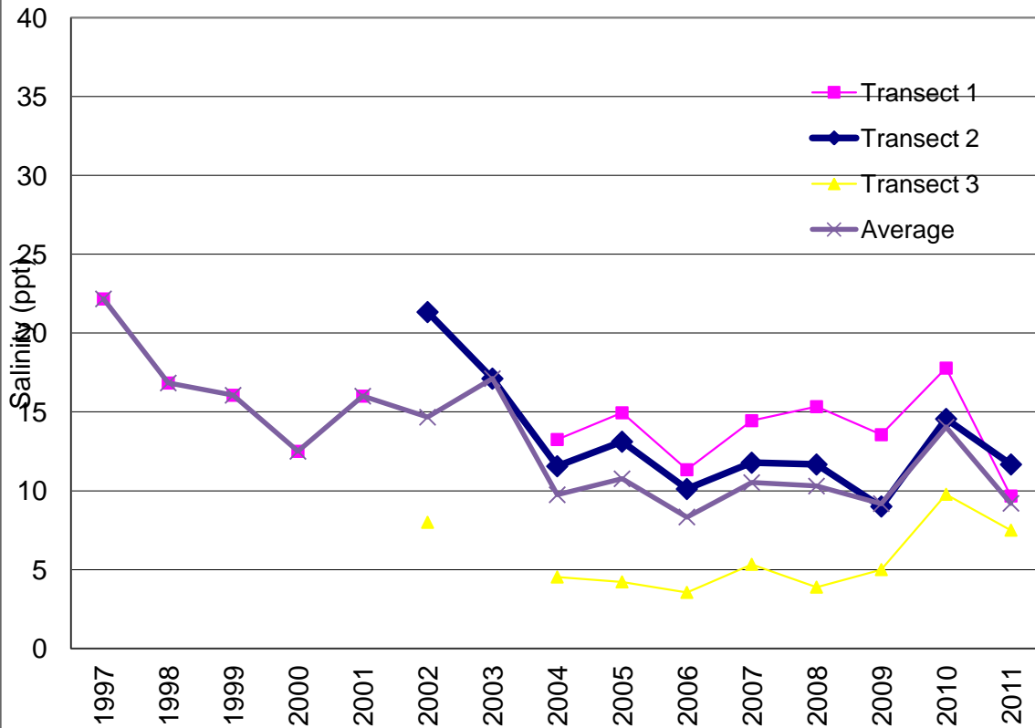
Rowley Salinity Averages 1997-2010
