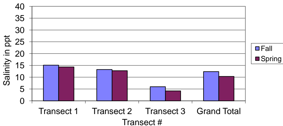
Seasonal Average Salinity by Transect, Batchelder's Landing, Rowley 1997-2011
