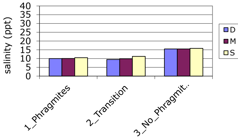
Railroad Ave., Rowley 1997-2011 Average Salinity vs. Presence of Phragmites and Well Depth
