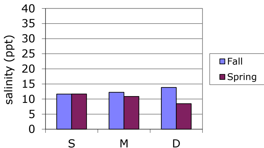
Railroad Ave., Rowley 1997-2011 Seasonal Average Salinity vs. Depth
