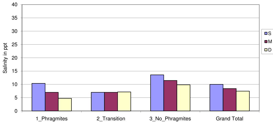
Cedar Point, Ipswich 1999-2001, 2004-2008 Average Salinity vs. Presence of Phragmites and Well Depth
