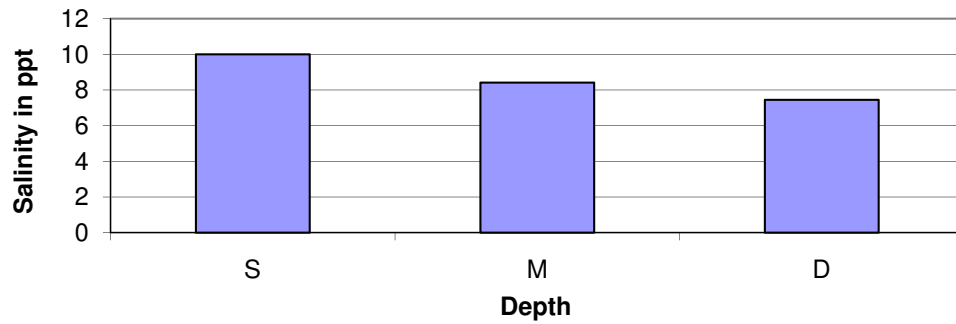
Cedar Point, Ipswich 1999-2001, 2004-2008 Average Salinity vs. Well Depth
