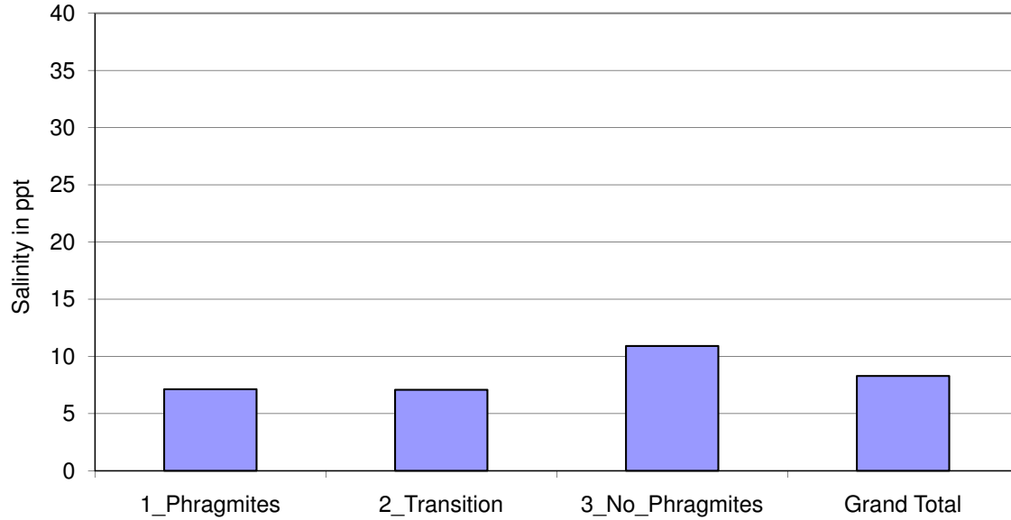
Cedar Point, Ipswich 1999-2001, 2008 Average Salinity vs. Presence of Phragmites
