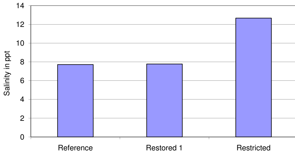
Cedar Point, Ipswich 1999-2001, 2004-2008 Average Salinity vs. Treatment Status
