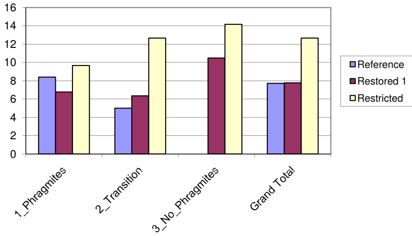
Average Salinity Comparison Pre and Post restoration Cedar Point, Ipswich
