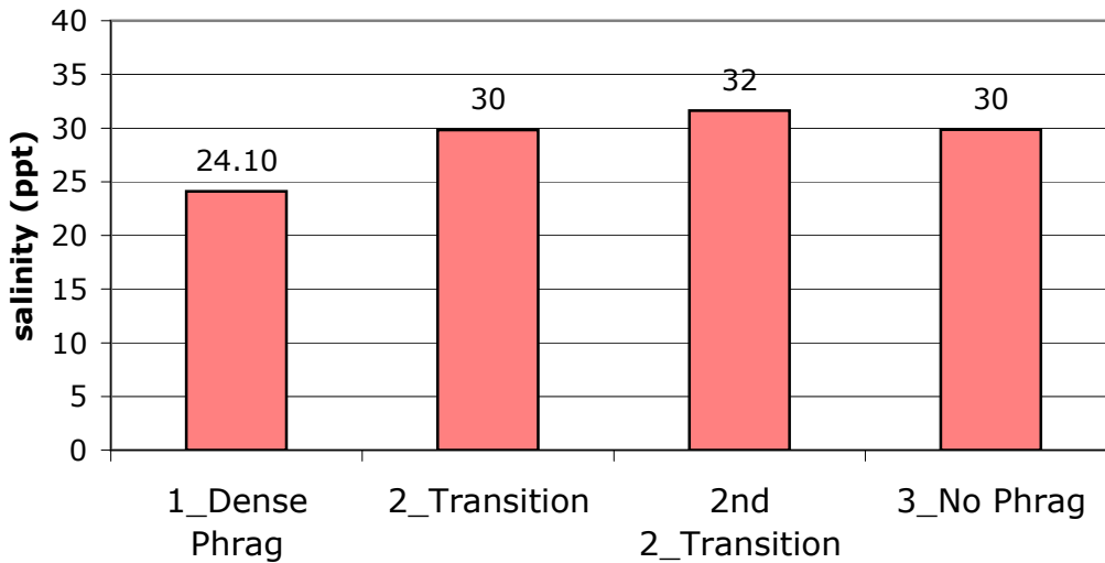
Osram Sylvania, Danvers 1998-2006 Average Salinity vs. Phragmites Density
