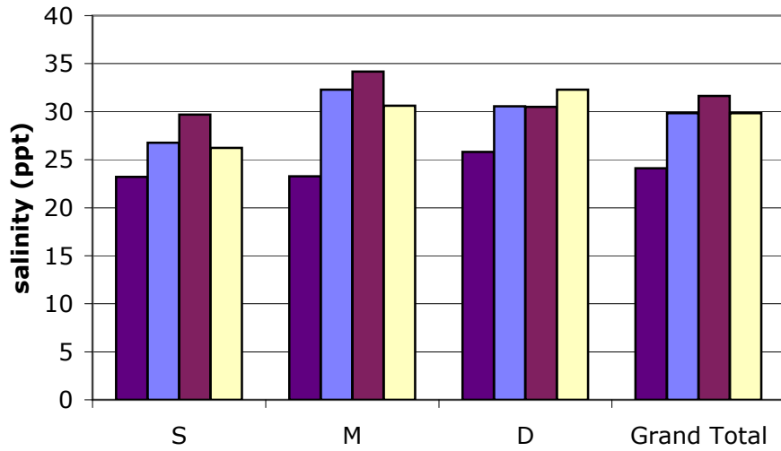
Osram Sylvania, Danvers 1998 - 2005 Average Salinity vs. Well Depth
